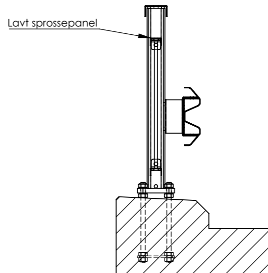
SECTION C-C SCALE 1 : 20
